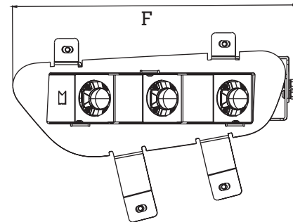
Bracket Dimension
