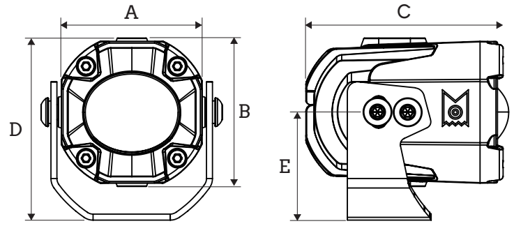
Lamp Dimension
