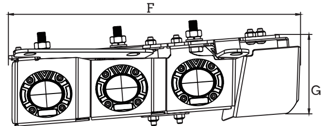
Bracket Dimension
